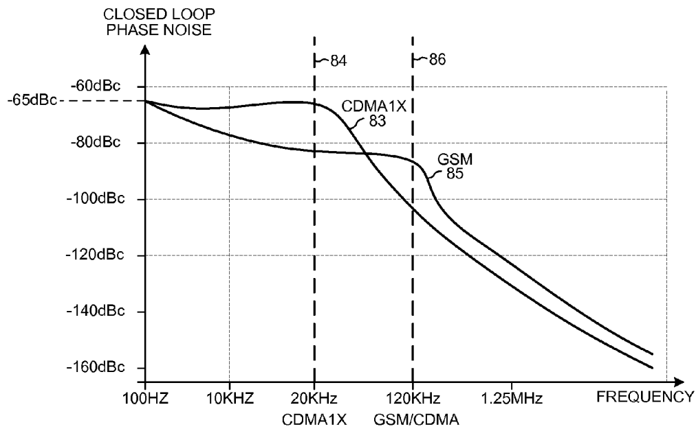
LOOP BANDWIDTH OF CLOSED LOOP PHASE NOISE
