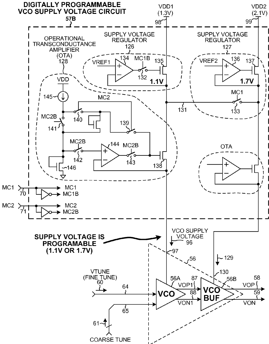
CASADED TWO-STAGE VCO SUPPLY VOLTAGE CIRCUIT
